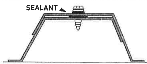
SIDE LAP
